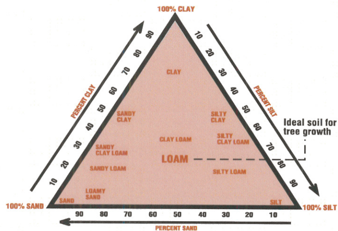
Figure 6. An ideal soil for tree growth is a mixture of sand, silt, clay, and organic matter, called loam.
